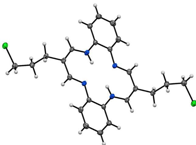
Figure 11. X-ray crystal structure of dctaa. Thermal ellipsoids shown at 50% probability level.
