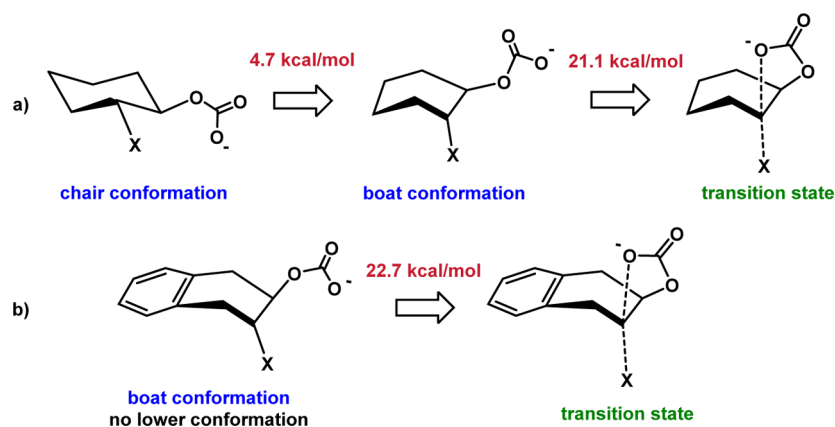
Figure 9. Schemed representations: (a) Total energetic barrier of 25.8 kcal/mol for carbonate backbiting of PCHC from its lowest energy chair conformation. (b) With the boat conformation as the energy minimum, PDNC has a lower backbiting barrier of 22.7 kcal/mol. Free energies calculated using the CBS-QB3 composite method. 6 The anionic polymer chain, X, is modeled as methyl carbonate.
